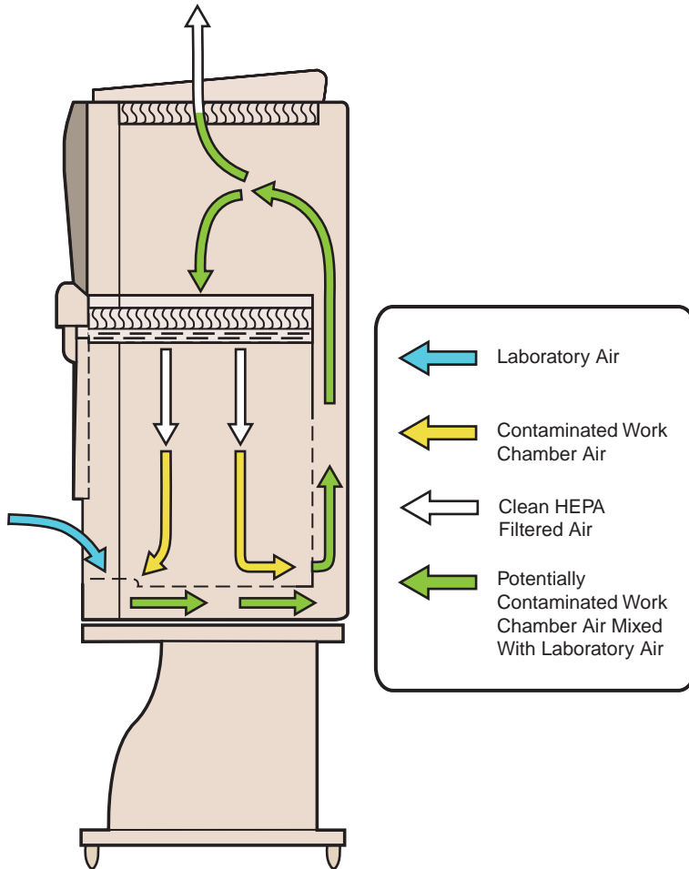
FIGURE 7.1. Class II, Type A2 Biological Safety Cabinet. (Courtesy of Microzone Corp., Ottawa, Ontario, Canada)
